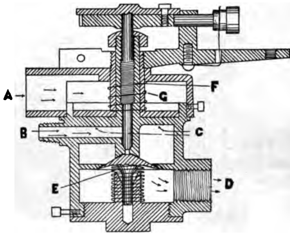
FIG. 166.—Sectional Diagram of the Haynes-Apperson Throttling Mixer. A, air inlet; B, gasoline inlet; C, C, location of air ports into mixing chamber; D, vapor exit to engine; E, mushroom valve held on seat by spring, opened by suction of engine piston; F, threaded needle valve spindle; G, spring for raising upper member of air chamber when released by screw motion of the levers attached to cover retaining screw and needle valve spindle, both being raised or lowered by the same movement.
